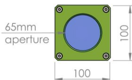
3" Window
